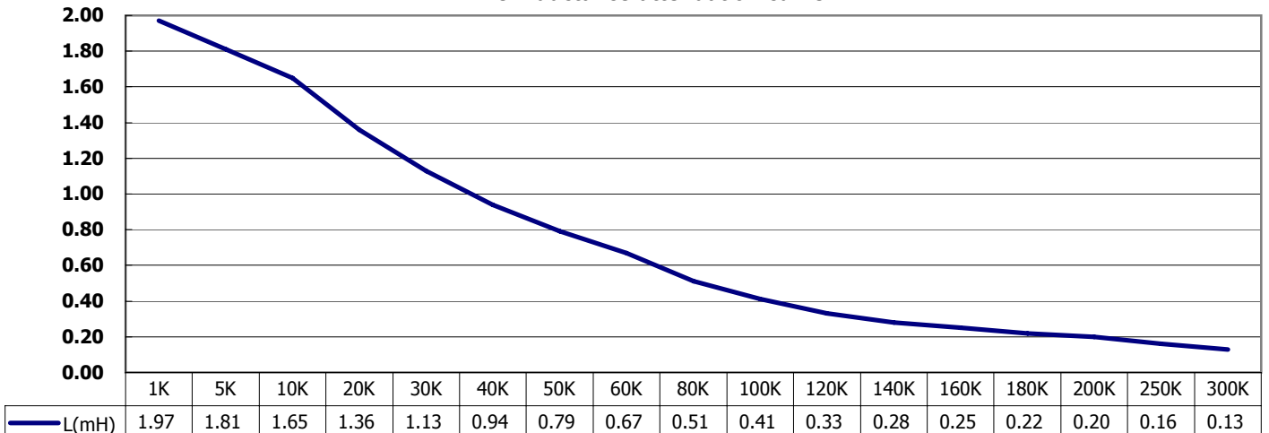
The inductance attenuation curve
