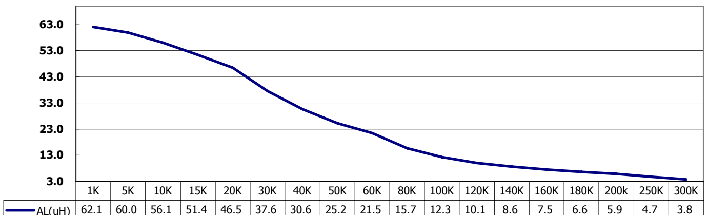
The inductance attenuation curve
