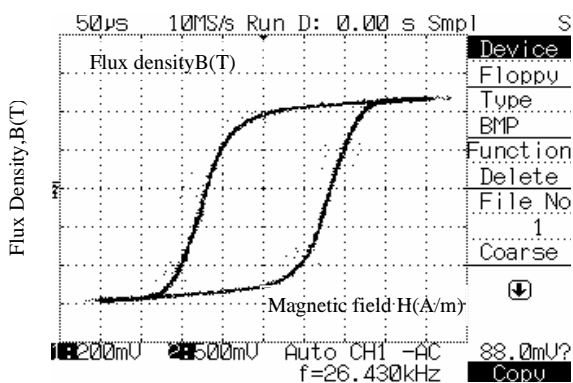
Hysteresis loops of core materials
