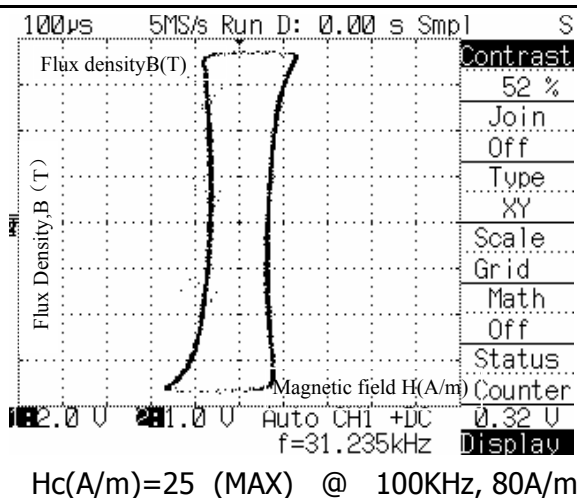
Hysteresis loops of core materials
